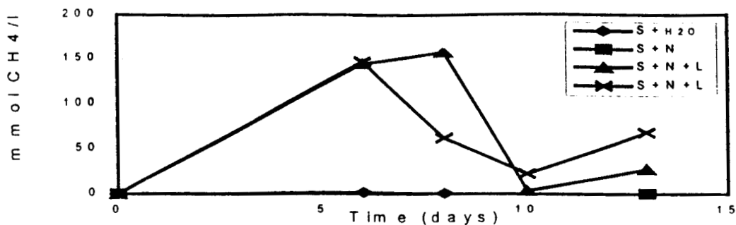
Figure 1. Production of CH 4 under anaerobic conditions. S+H 2 O, contaminated soil and water; S+N, contaminated soil and nutrients; S+N+L, contaminated soil, nutrients and sludge.
